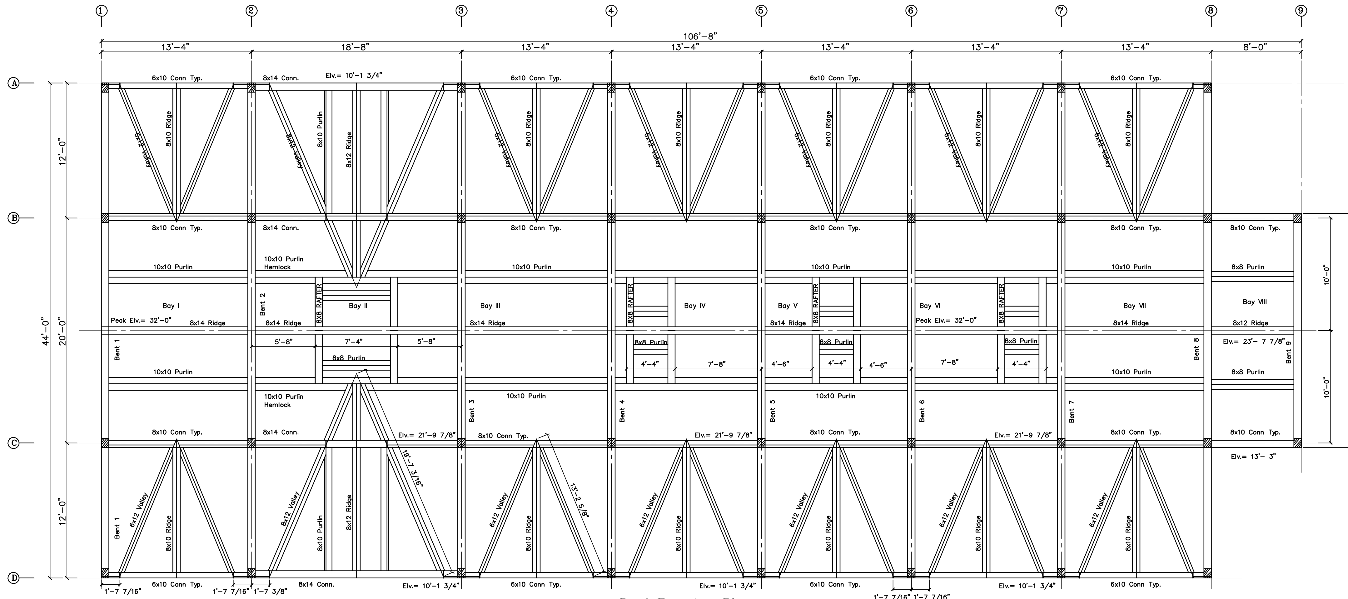
Roof Framing Plan
