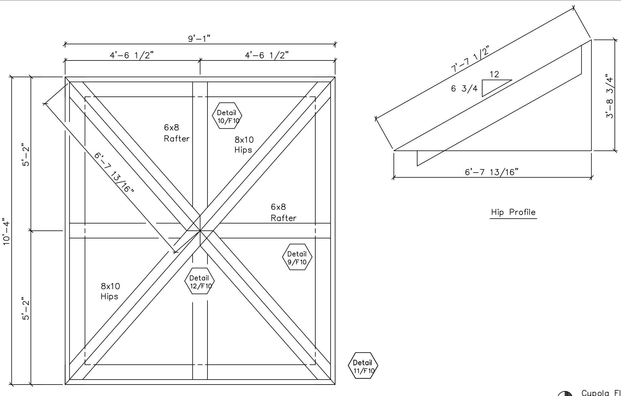
Cupola Roof Framing
