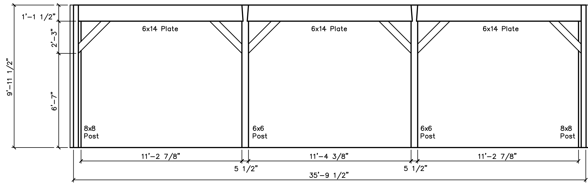
Porch Framing
