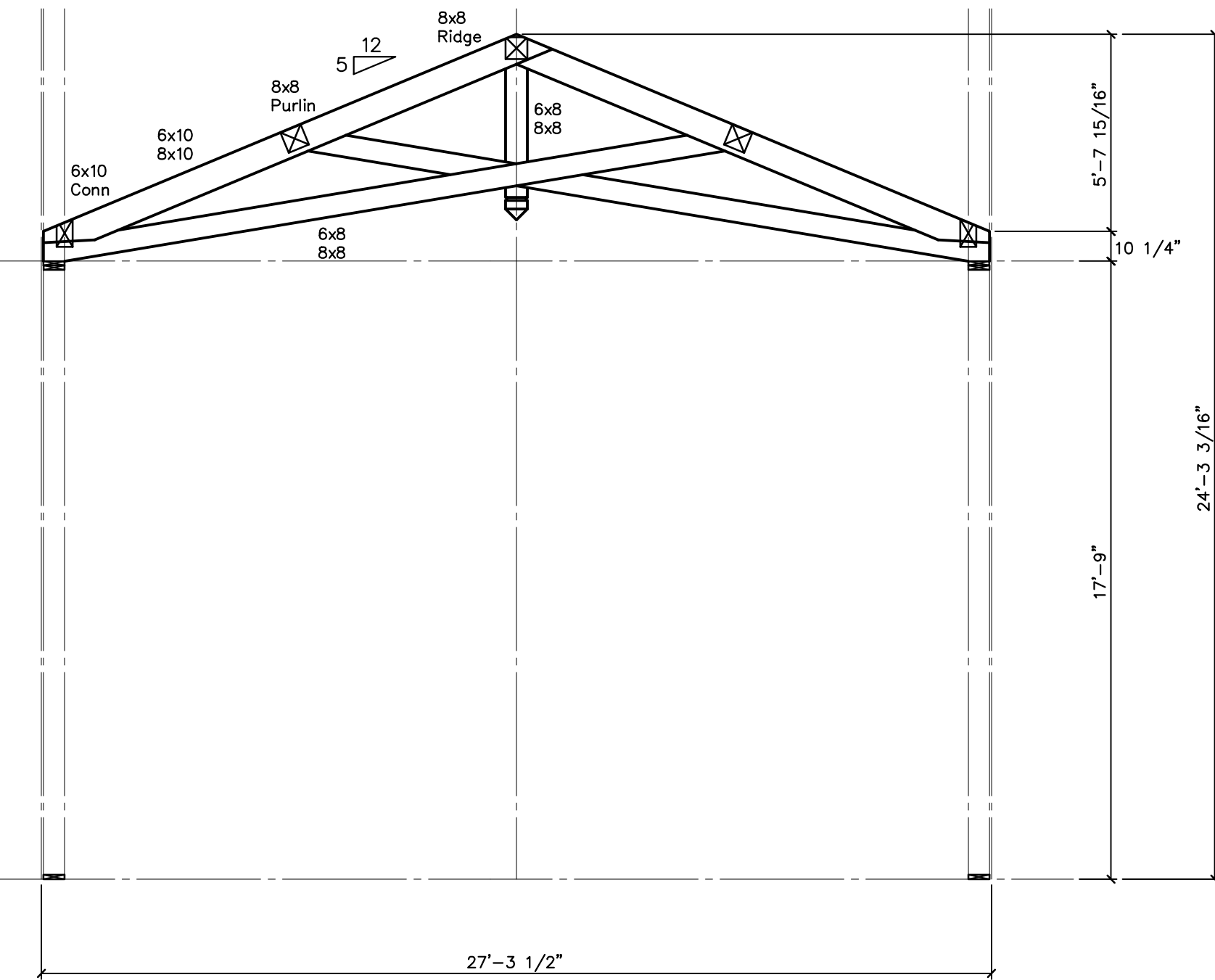
Alter Truss
