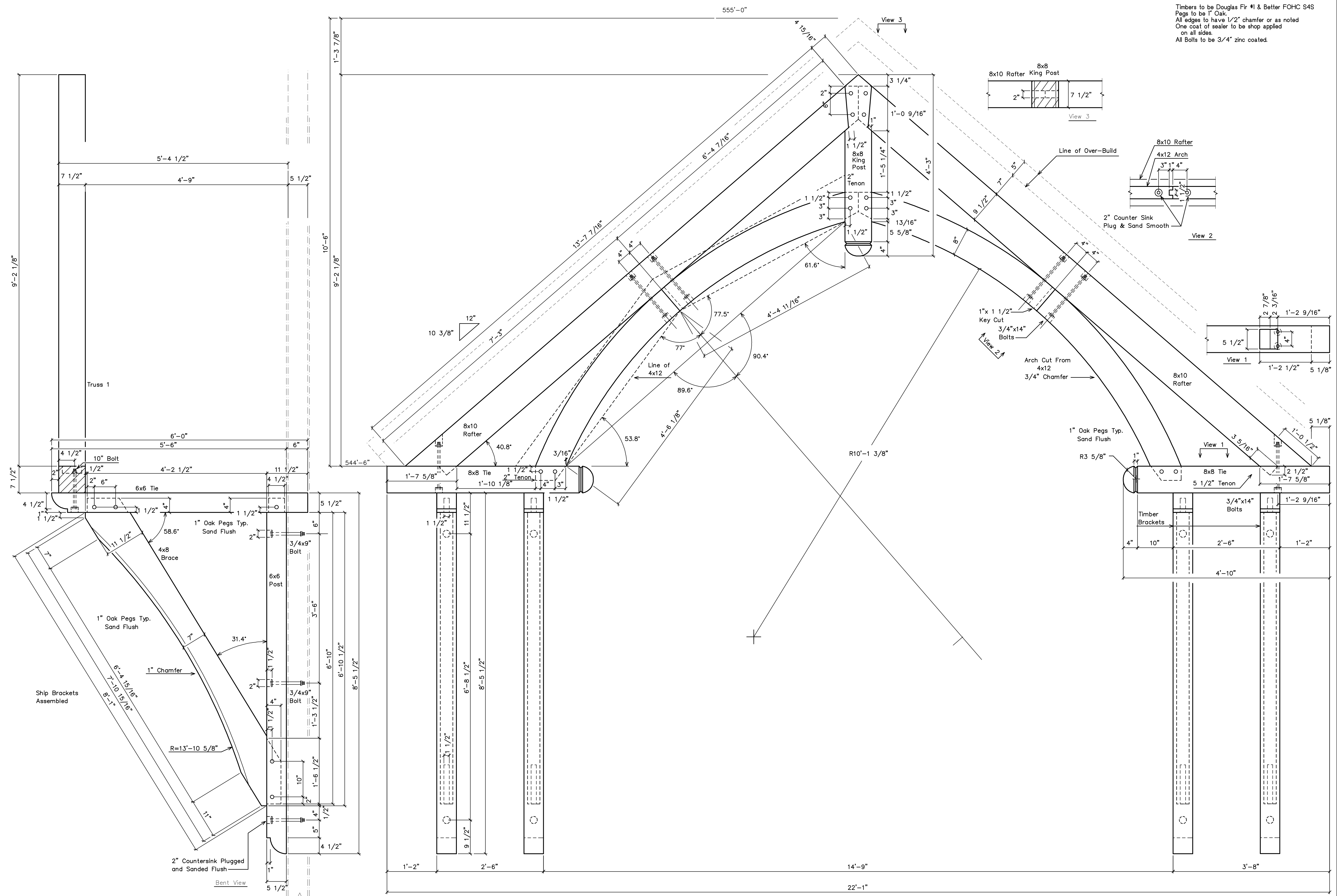
1 Canopy Bracket at Entry F-1 From Detail 2/A-8 - 4 Braces Required
