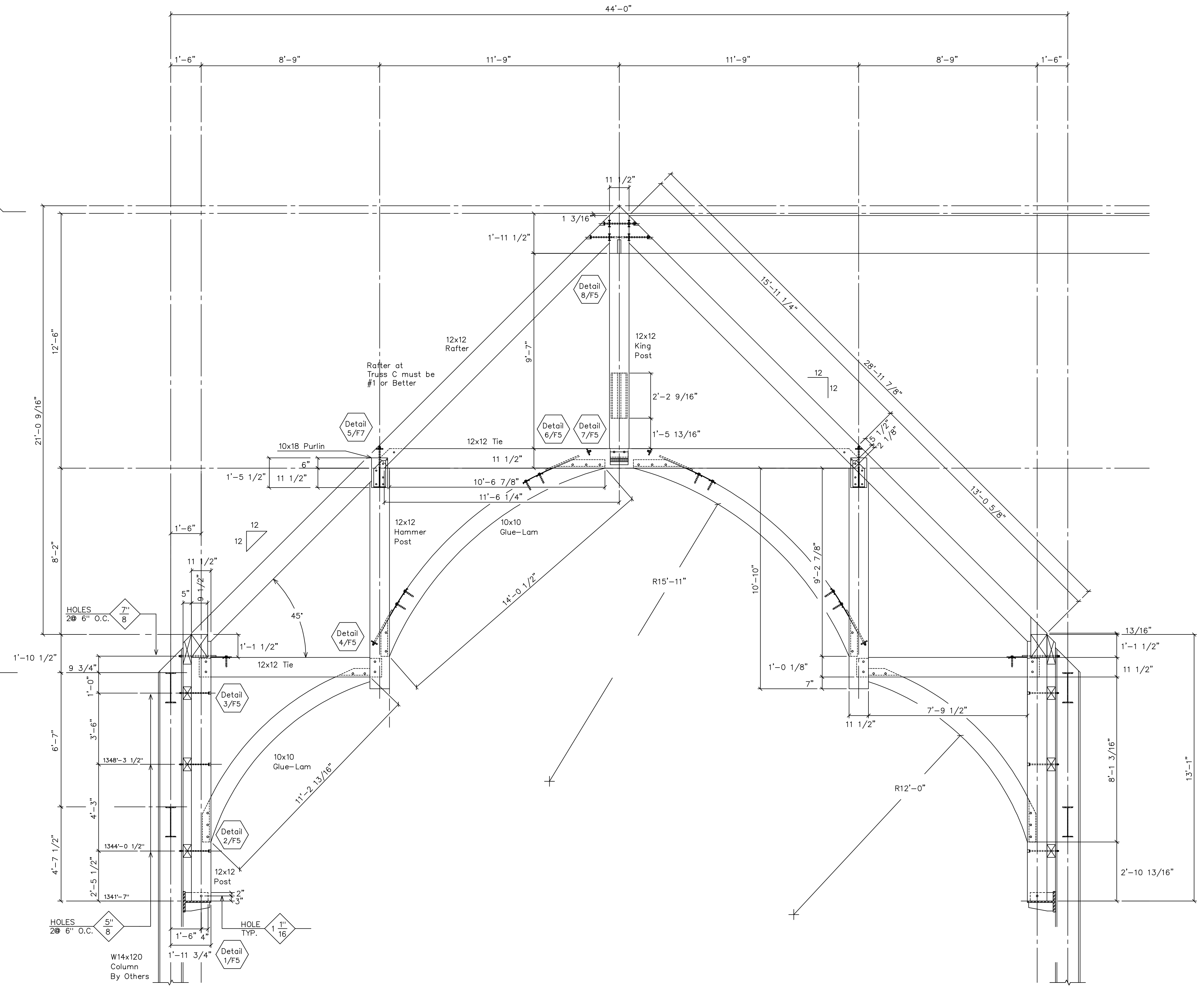
Truss C
