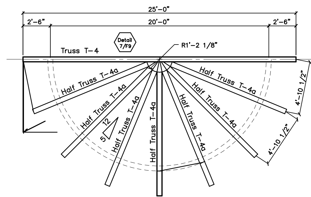
Turret Tie Framing
