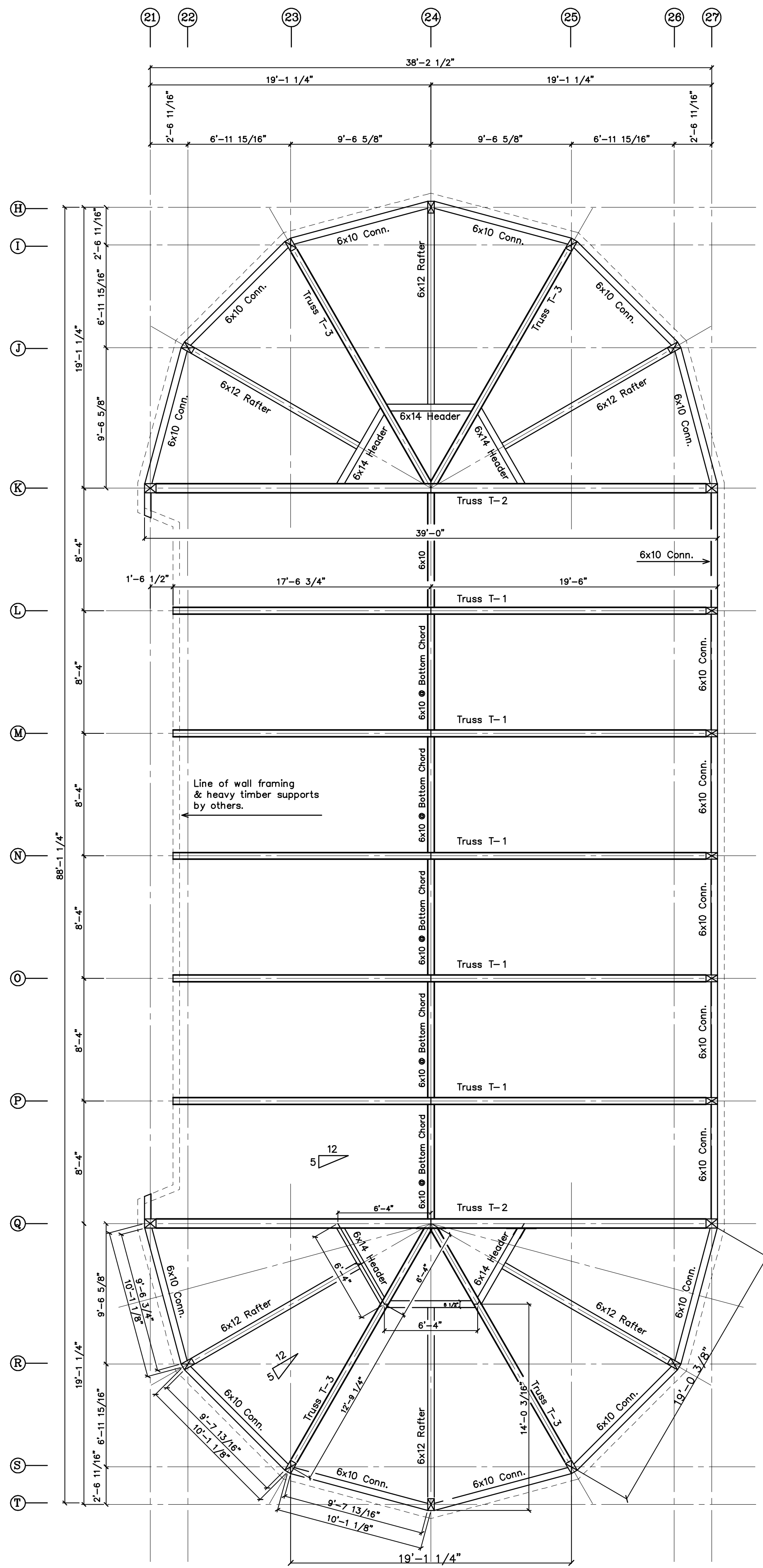
Pool Roof Framing
