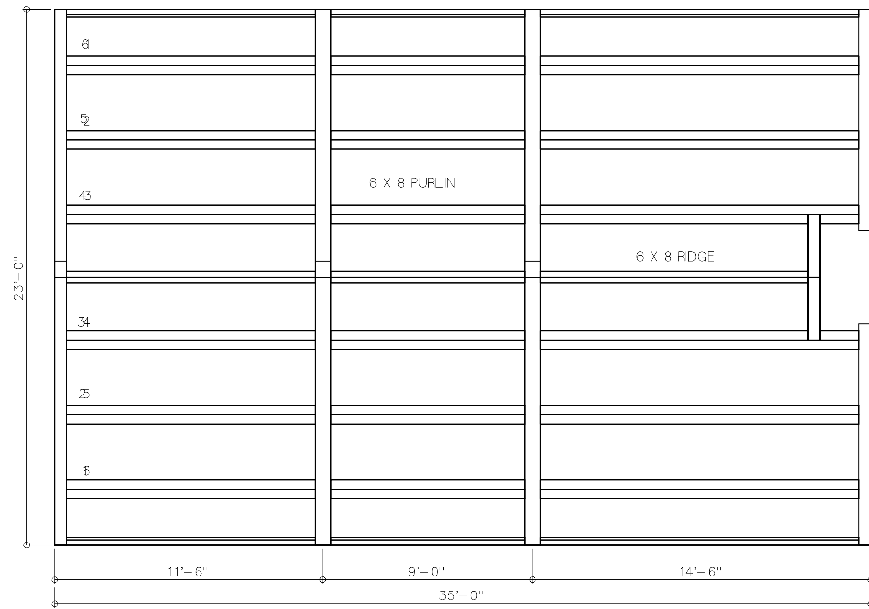
ROOF FRAMING
