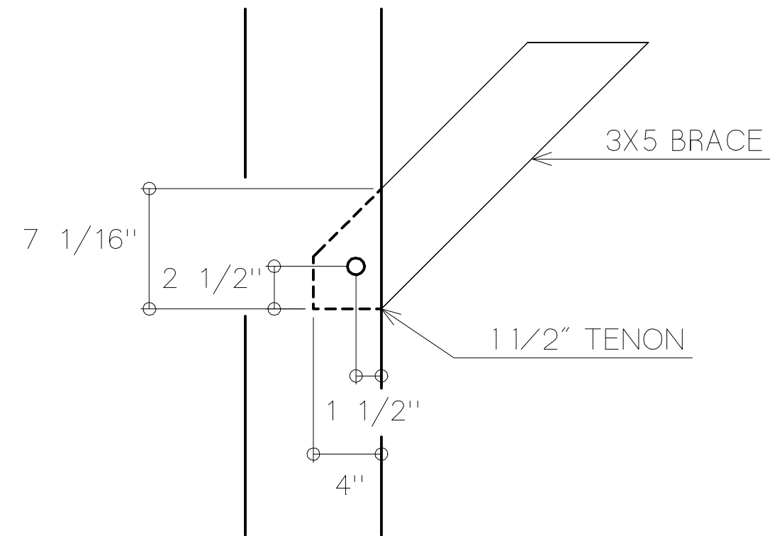
TYPICAL BRACE
