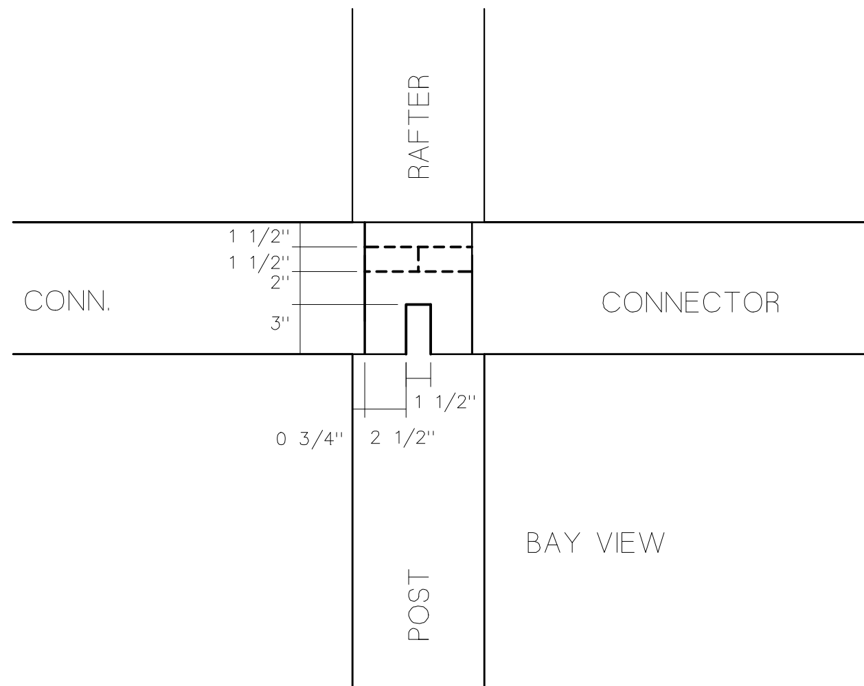
RAFTER FOOT WITH 8X8 TIES AND CONNECTOR
