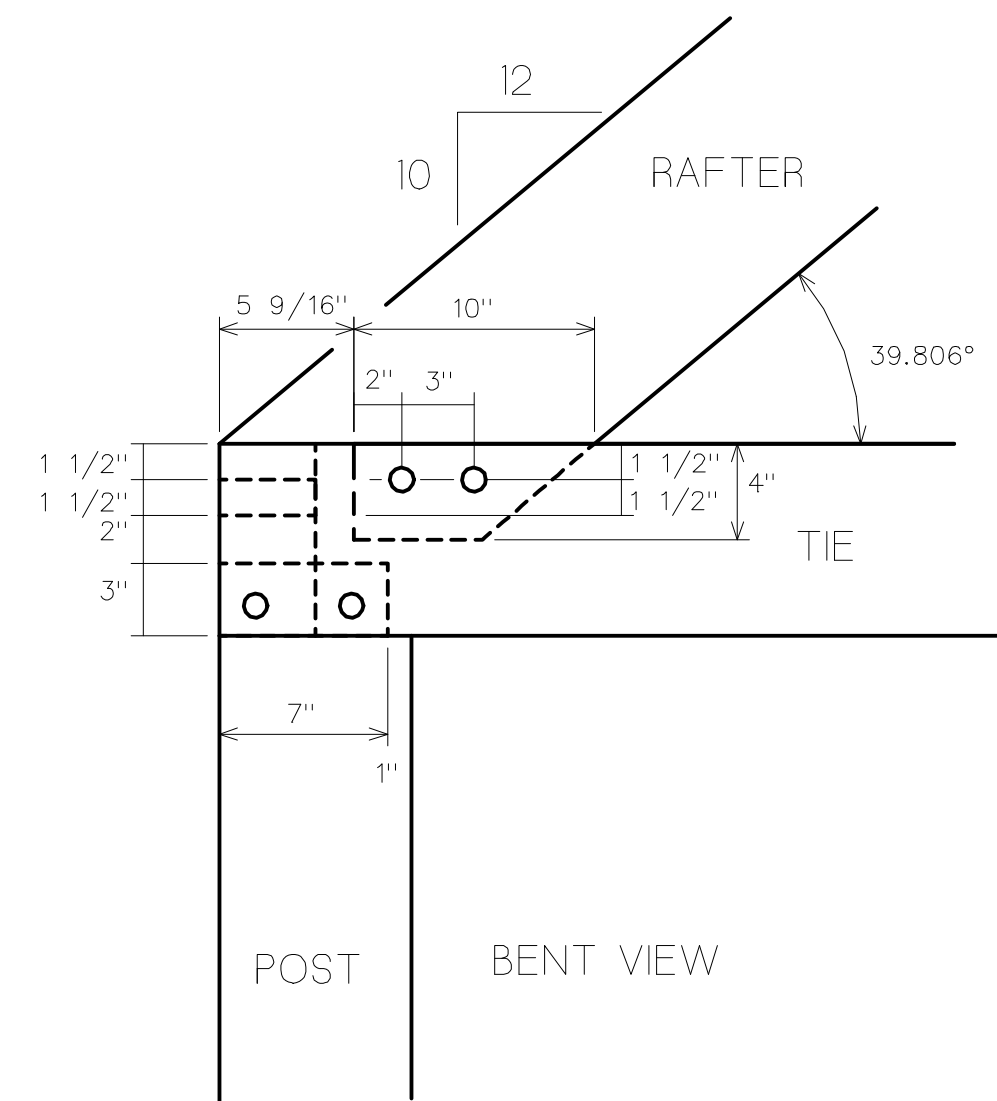
RAFTER FOOT WITH 8X8 TIES AND CONNECTOR
