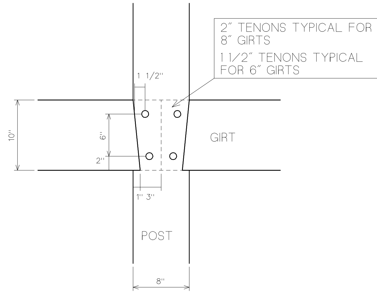
TYPICAL DOVETAIL
