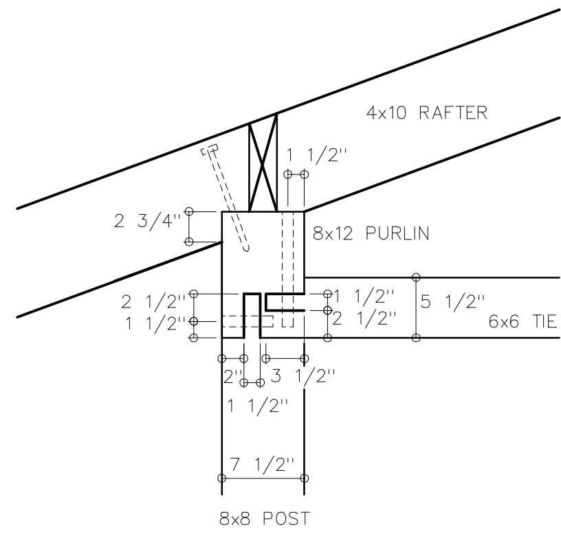
RAFTER AT BENT 2, POST A
